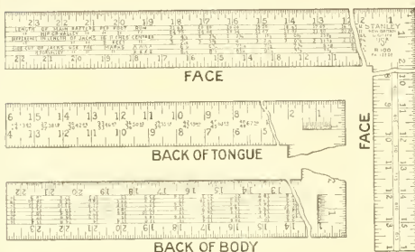
Stanley Steel Square.
